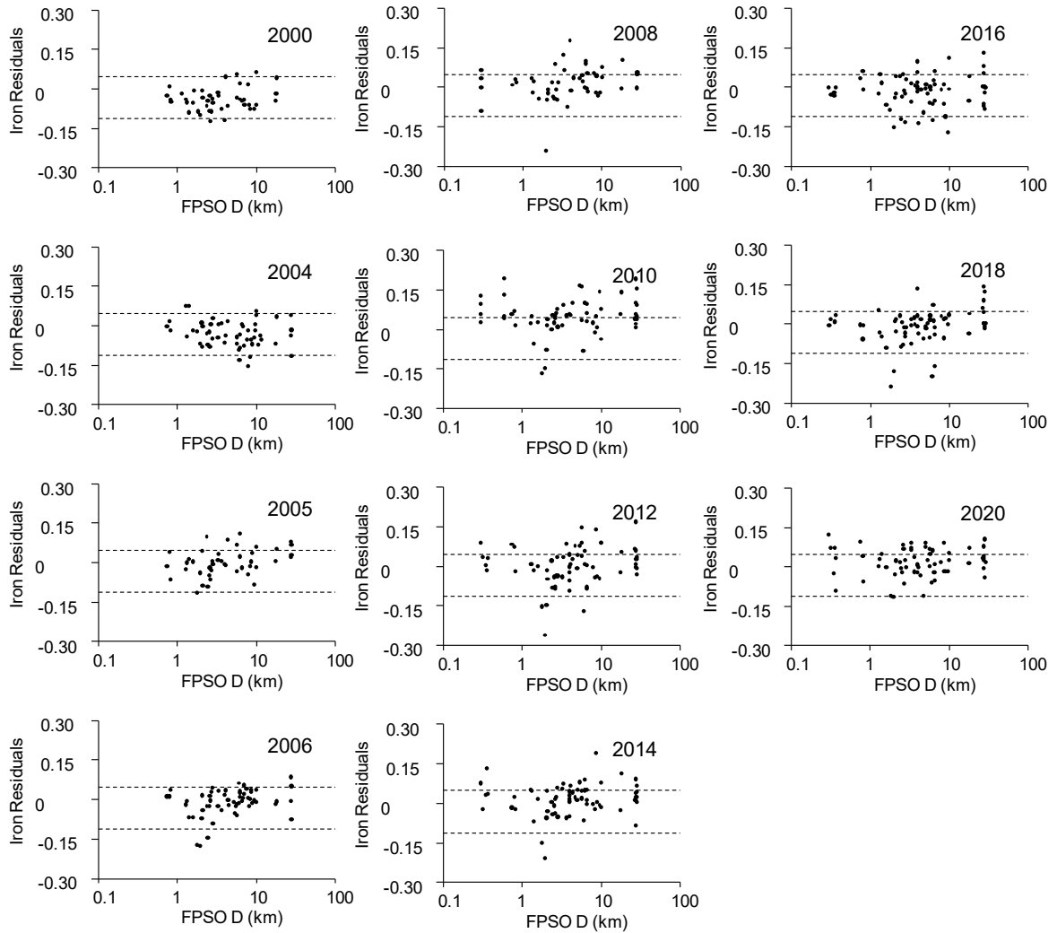
Figure 7-7 Variation in Iron Residuals with Distance from the SeaRose FPSO (FPSO D) (all Years)
