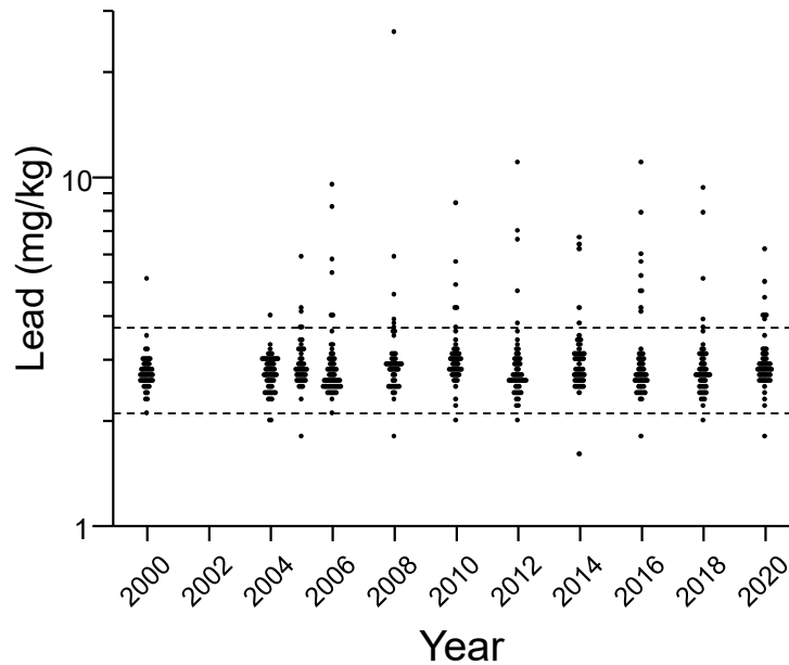
Figure 5-39 Dot Density Plot of Lead by Year
