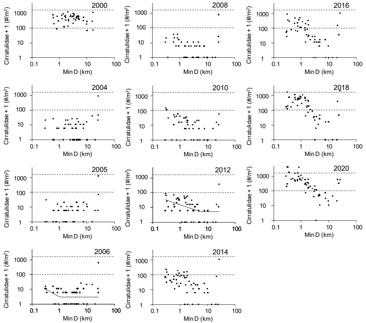
Figure 5-65 Variation in Cirratulidae Abundance (#/m 2 ) with Distance from Nearest Active Drill Centre (all Years)
